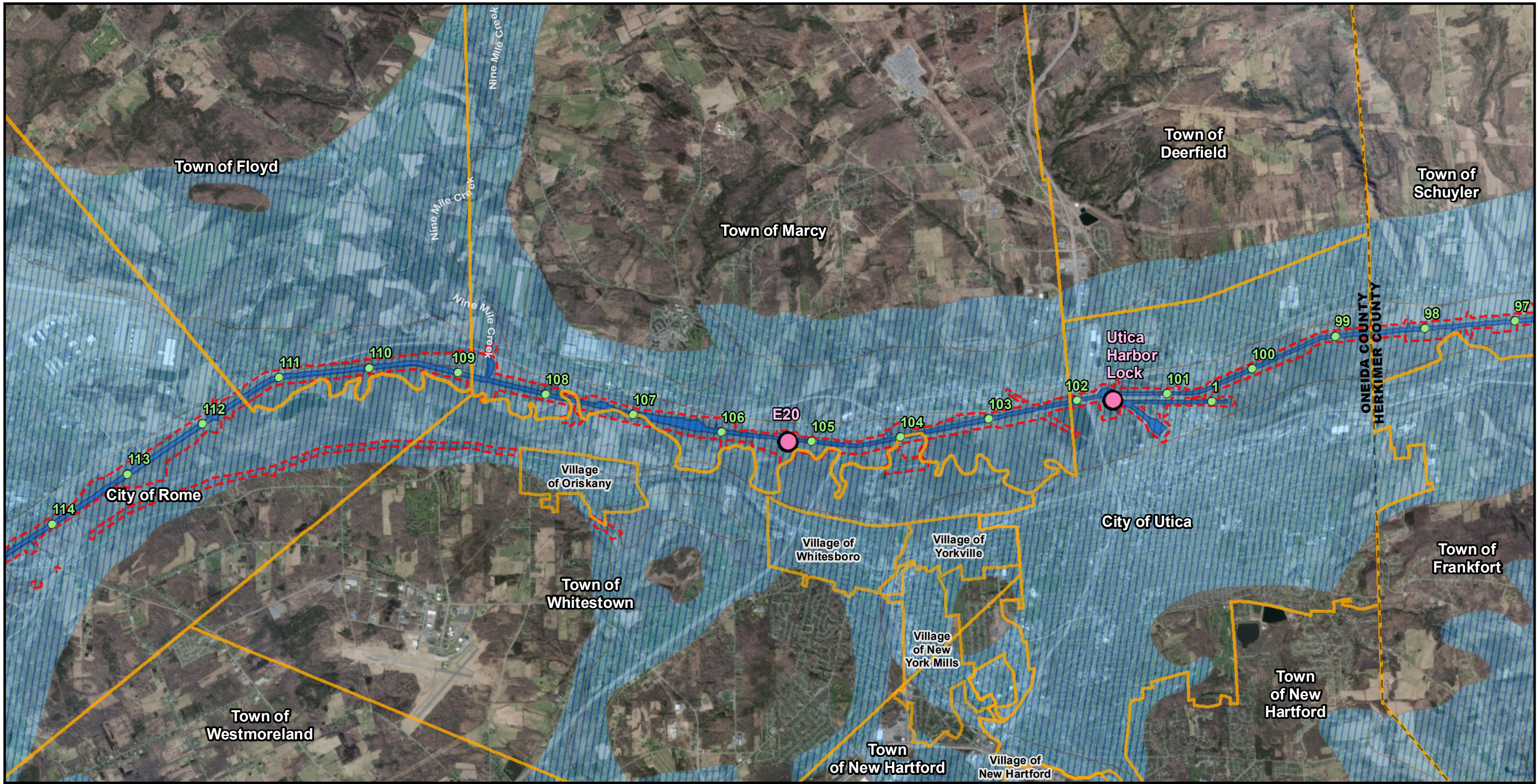
Figure 46F: Aquifers
